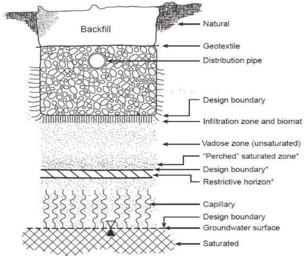
Figure 5-3. Subsurface wastewater infiltration system design/performance boundaries.
